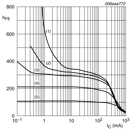
V_{CE} = 5\text{ V} (1) T_{amb} = 150\text{ }^\circ\text{C} (2) T_{amb} = 125\text{ }^\circ\text{C} (3) T_{amb} = 100\text{ }^\circ\text{C} (4) T_{amb} = 25\text{ }^\circ\text{C} (5) T_{amb} = -55\text{ }^\circ\text{C}
